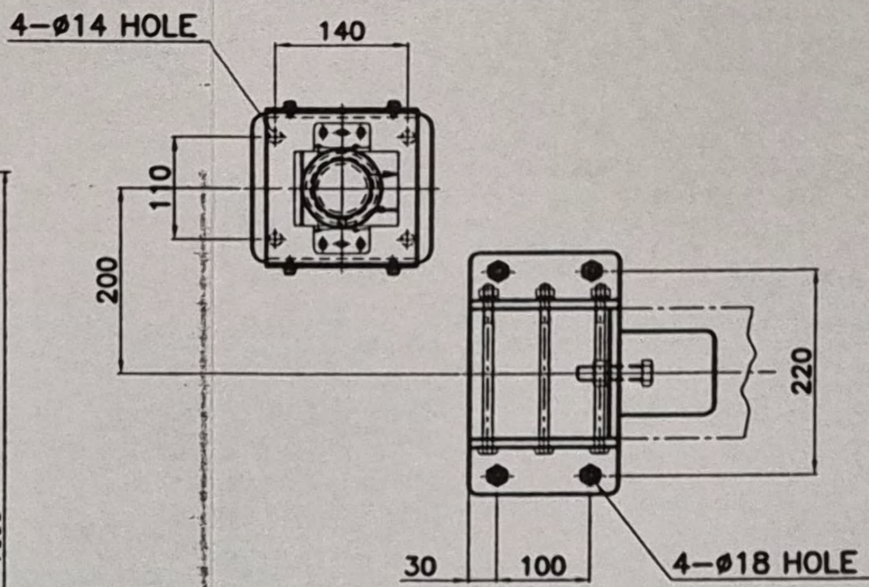
SENSOR ARRANGEMENT (SCALE 10/1)
