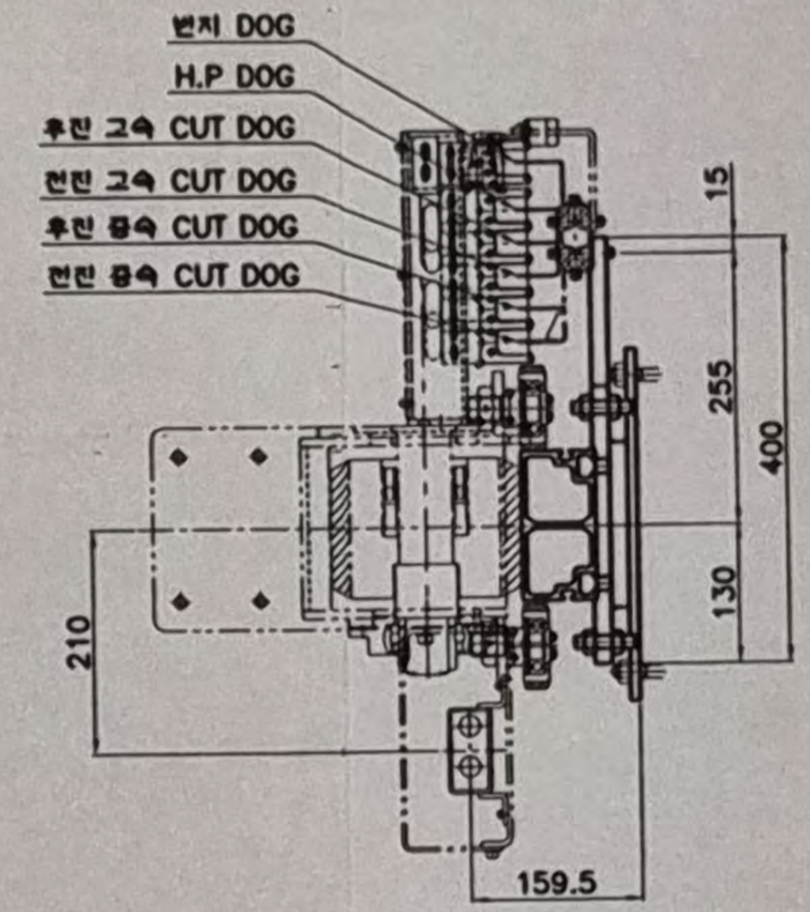
SENSOR ARRANGEMENT (SCALE 10/1)
