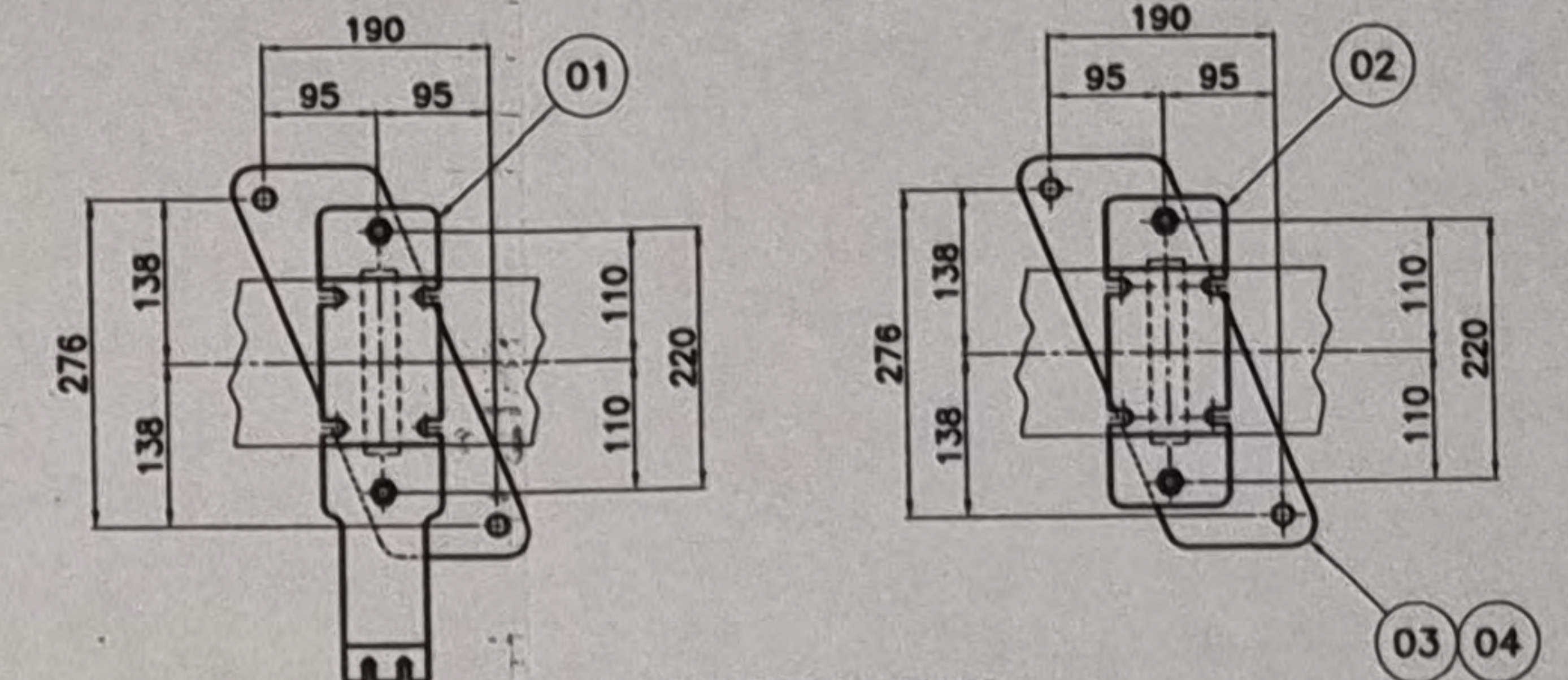
ANCHOR DETAIL (SCALE 10/1)
