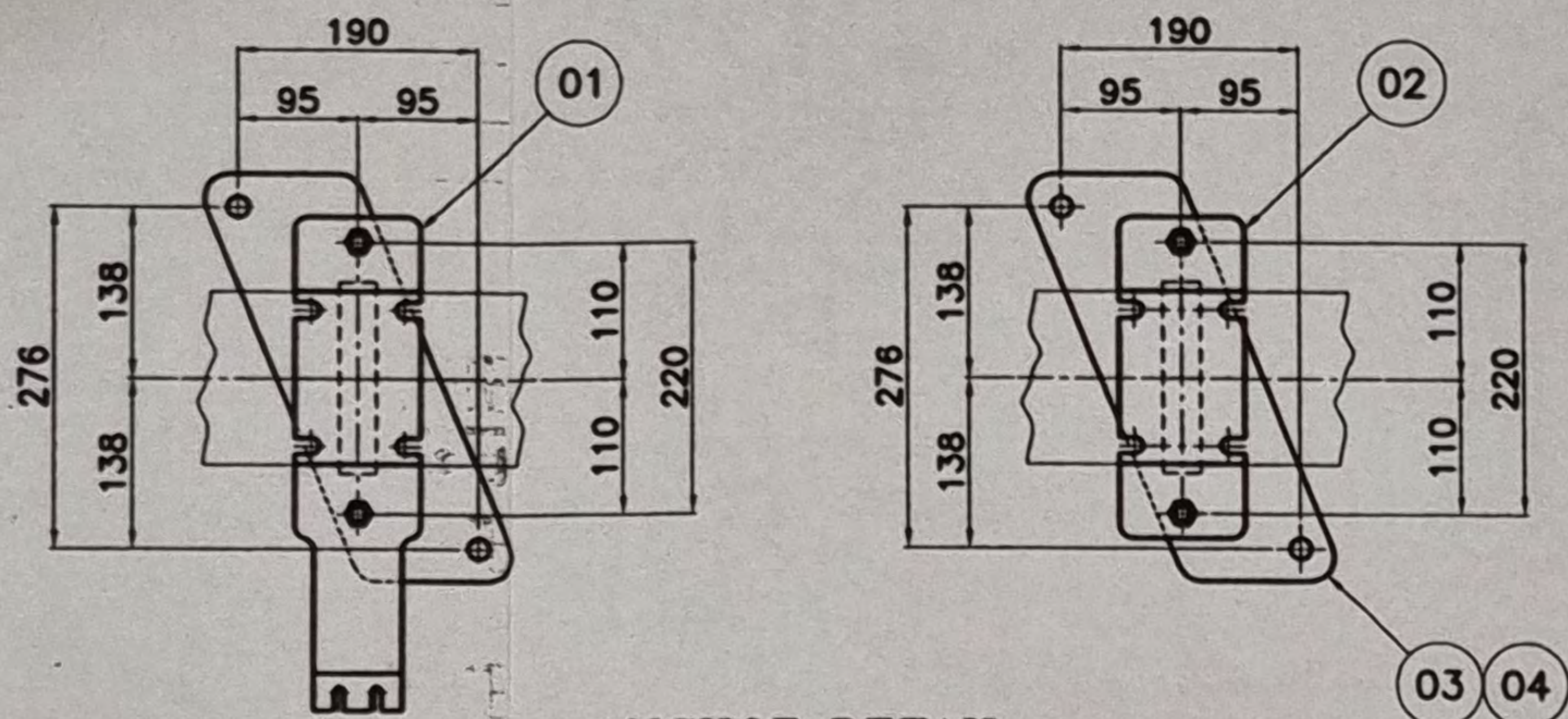
ANCHOR DETAIL (SCALE 10/1)
