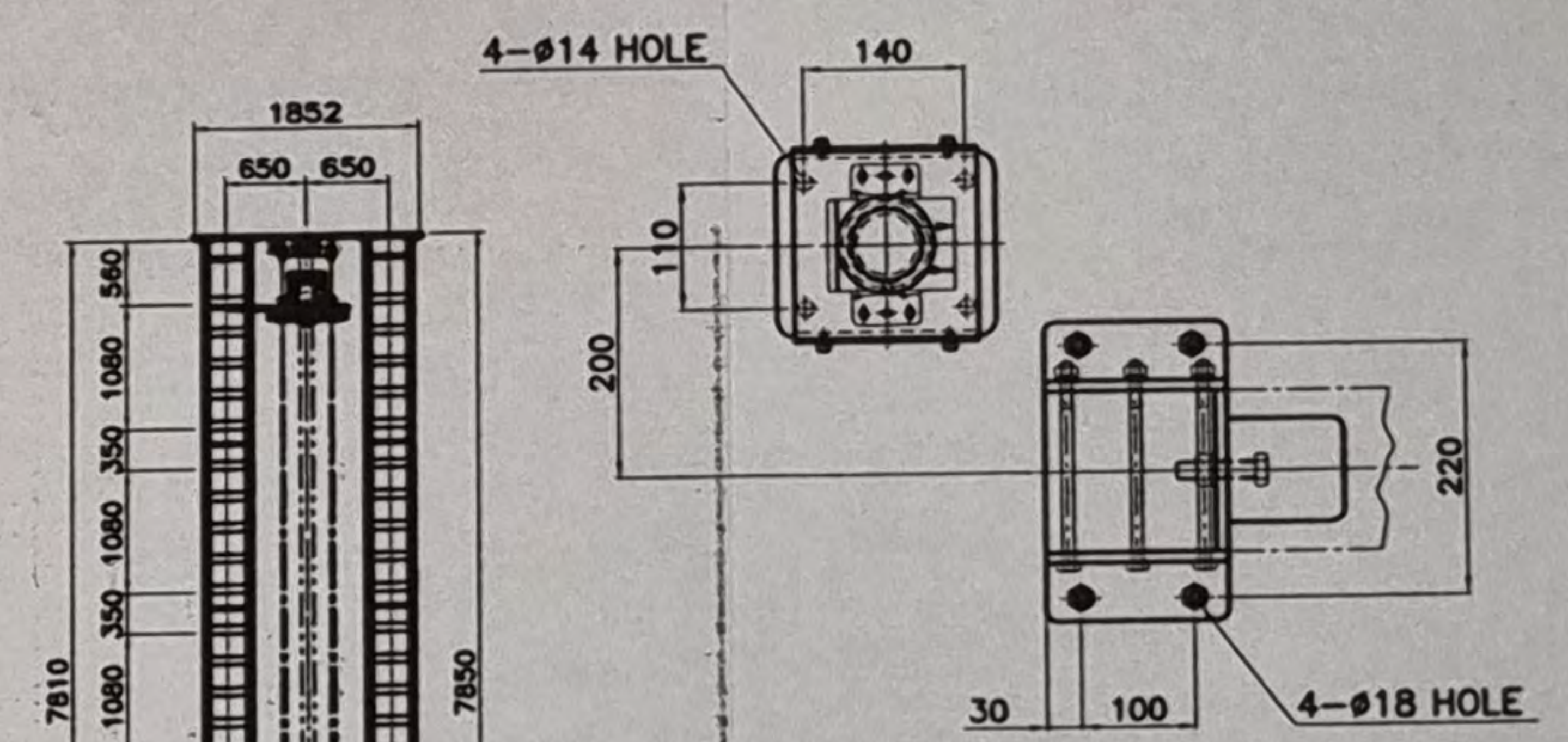
SENSOR ARRANGEMENT (SCALE 10/1)
